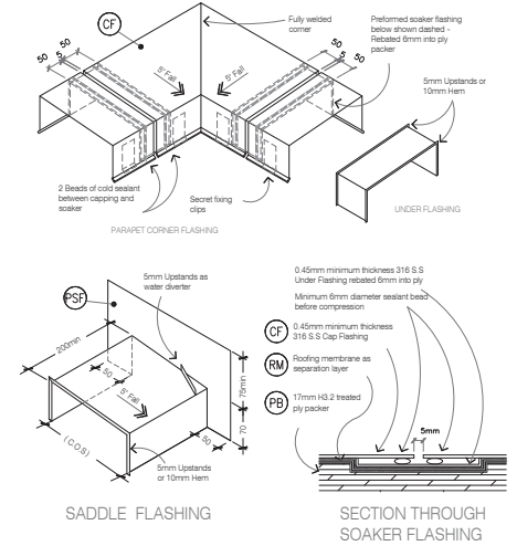
TYPICAL PARAPET CAPPING JOINT DETAILS Cavity Fix - Bevel Back WB SCALE 1:5 @ A1, 1:10 @ A3
