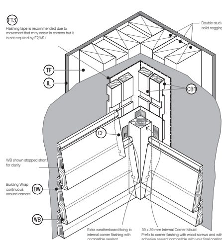
C17 3D INTERNAL CORNER - J101 BC61 Cavity Fix - Bevel Back WB SCALE : N.T.S
