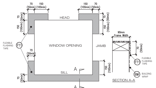
W5 FLEXIBLE BUILDING WRAP AT OPENING SCALE : 1 / 2 @ A1, 1 / 10 @ A3
