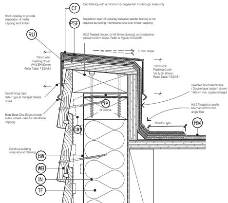
PARAPET SECTION TO MEMBRANE ROOF Cavity Fix - Bevel Back WB SCALE 1:2.5 @ A1, 1:5 @ A3
