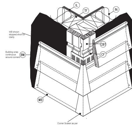
C13 3D EXTERNAL CORNER - SOAKER BC53 Cavity Fix - Bevel Back WB SCALE : N.T.S
