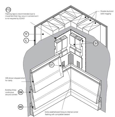
C19 3D INTERNAL CORNER BC63 Cavity Fix - Bevel Back WB SCALE : N.T.S
