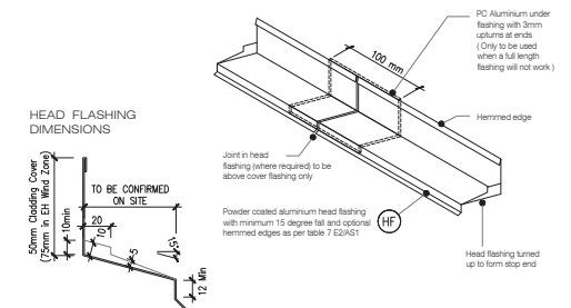
D6 TYPICAL HEAD & FLASHING JOINT BC23 SCALE : 1 / 2 @ A1, 1 / 4 @ A3
