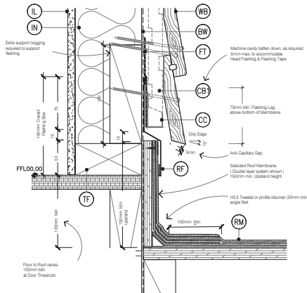
BASE OF WALL, MEMBRANE ROOF Cavity Fix - Bevel Back WB SCALE 1:2.5 @ A1, 1:5 @ A3
