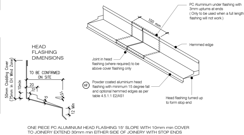
W6 TYPICAL HEAD & FLASHING JOINT SCALE : 1 / 2 @ A1, 1 / 4 @ A3
