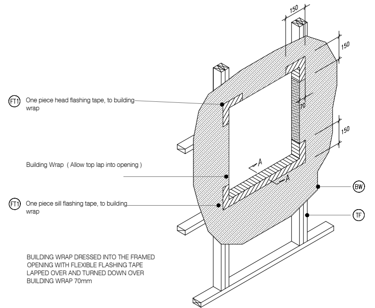
M4 TYPICAL METER BOX OPENING ( FLASHING TAPE ) BB33 SCALE : N.T.S
