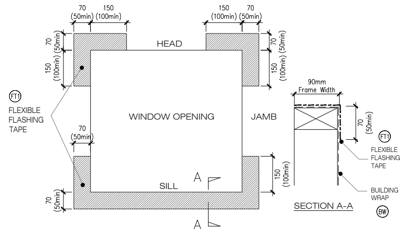
W5 FLEXIBLE BUILDING WRAP AT OPENING SCALE : 1 / 5 @ A1, 1 / 10 @ A3
