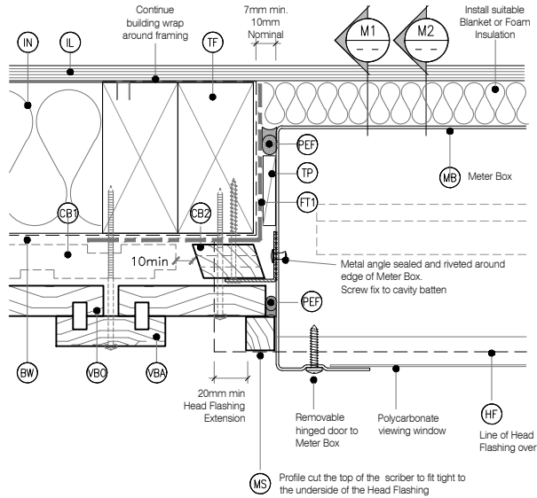
M3 METER BOX JAMB BB32 Cavity Fix - Board & Batten System SCALE 1:2 @ A1, 1:4 @ A3
