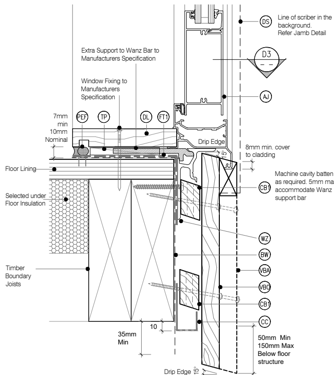
D2 DOOR SILL - Board & Batten System BB21 Cavity Fix - Aluminium Joinery - Double Glazing SCALE 1:2 @ A1, 1:4 @ A3
