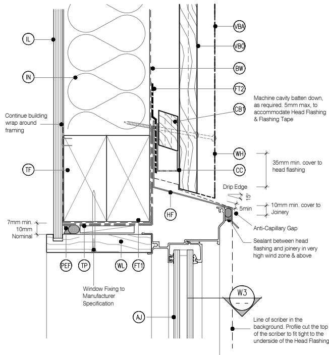
W1 WINDOW HEAD - Board & Batten System Cavity Fix - Aluminium Joinery - Double Glazing SCALE 1:2 @ A1, 1:4 @ A3
