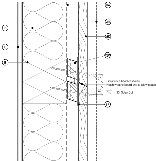
C2 WEATHERBOARD SCARF JOINT BB41 Cavity Fix - Board & Batten System SCALE 1:2 @ A1, 1:4 @ A3
