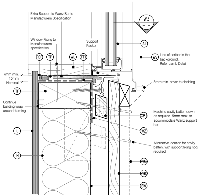
W2 WINDOW SILL - Board & Batten System Cavity Fix - Aluminium Joinery - Double Glazing SCALE 1:2 @ A1, 1:4 @ A3
