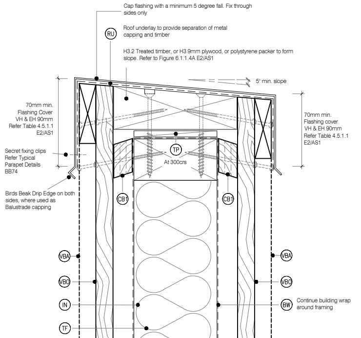
C21 BALUSTARDE CAPPING OR PARAPET DETAIL Cavity Fix - Board & Batten System SCALE 1:2 @ A1, 1:4 @ A3
