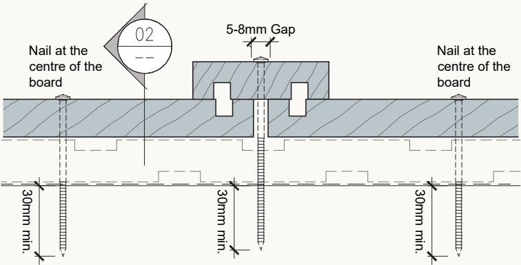
Plan Section 01
