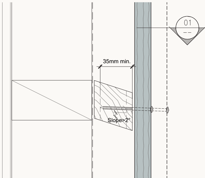
Cross Section 02
