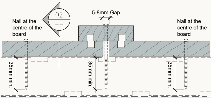
Plan Section 01
