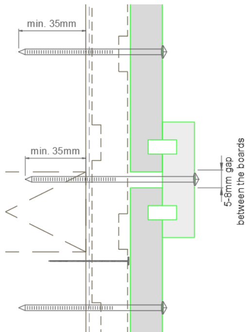
Figure 1 - Typical Board & Batten Weatherboard Installation
