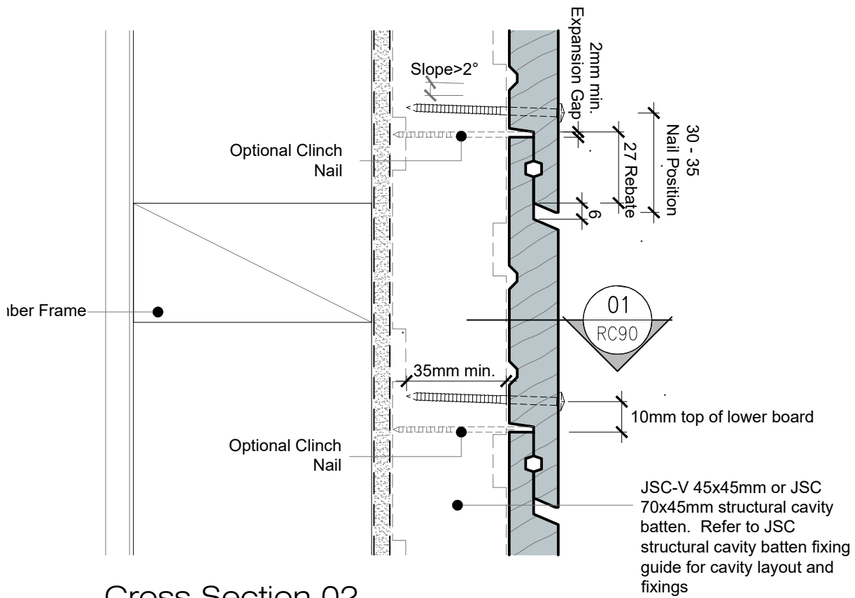
Cross Section 02
