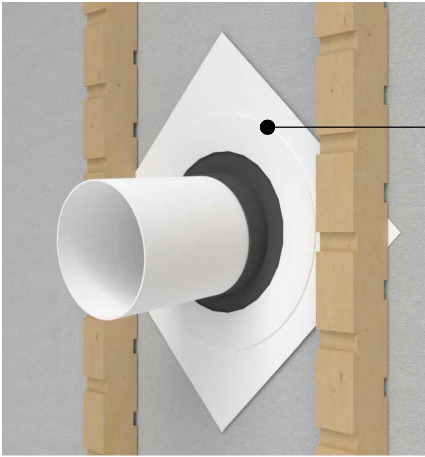
Solid blocking around penetration with min. 75mm overlap to underlay
