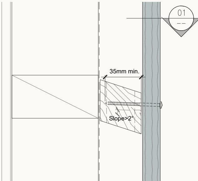
Cross Section 02
