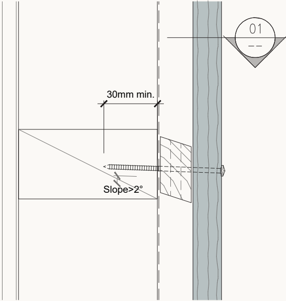
Cross Section 02
