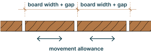
Fig. 1 - Boards layout
