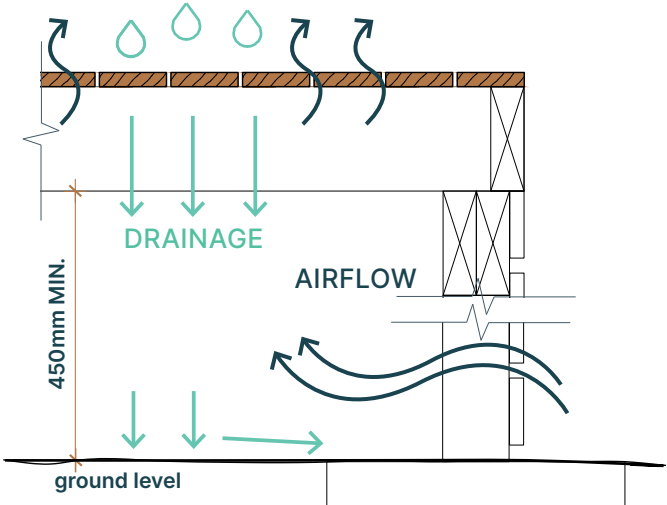
Fig. 2 - Ventilation and drainage
