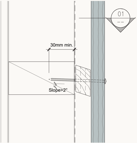
Cross Section 02
